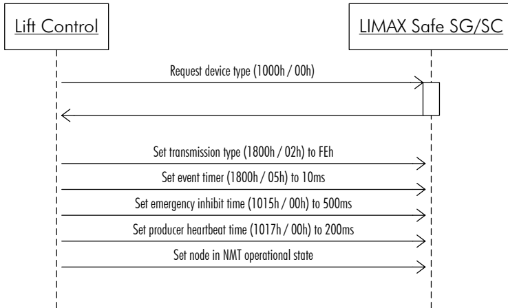
Fig. 19: Sequence diagram start-up (example)
